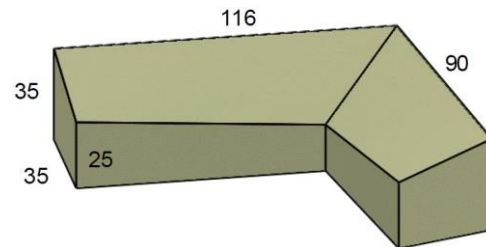
FC054 CABO SECTIONAL LEFT COVER LL, M, SCC90, RL FITS: 270, 275, 4302, 5306, 2685, 6400 W: 116/90" D: 35" H: 25/35"
