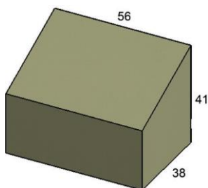
FC082 LOVESEAT COVER FITS: 3350, 4312, 4331, 4345 W: 56" D: 38" H: 41"
